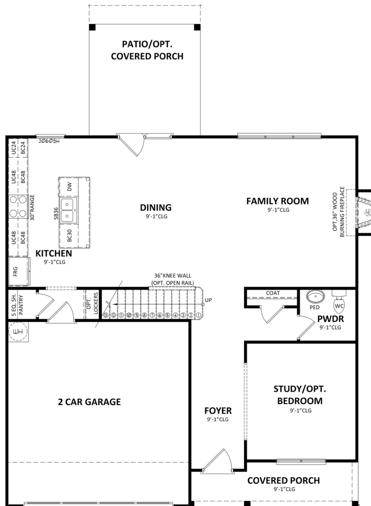
MAIN FLOOR
