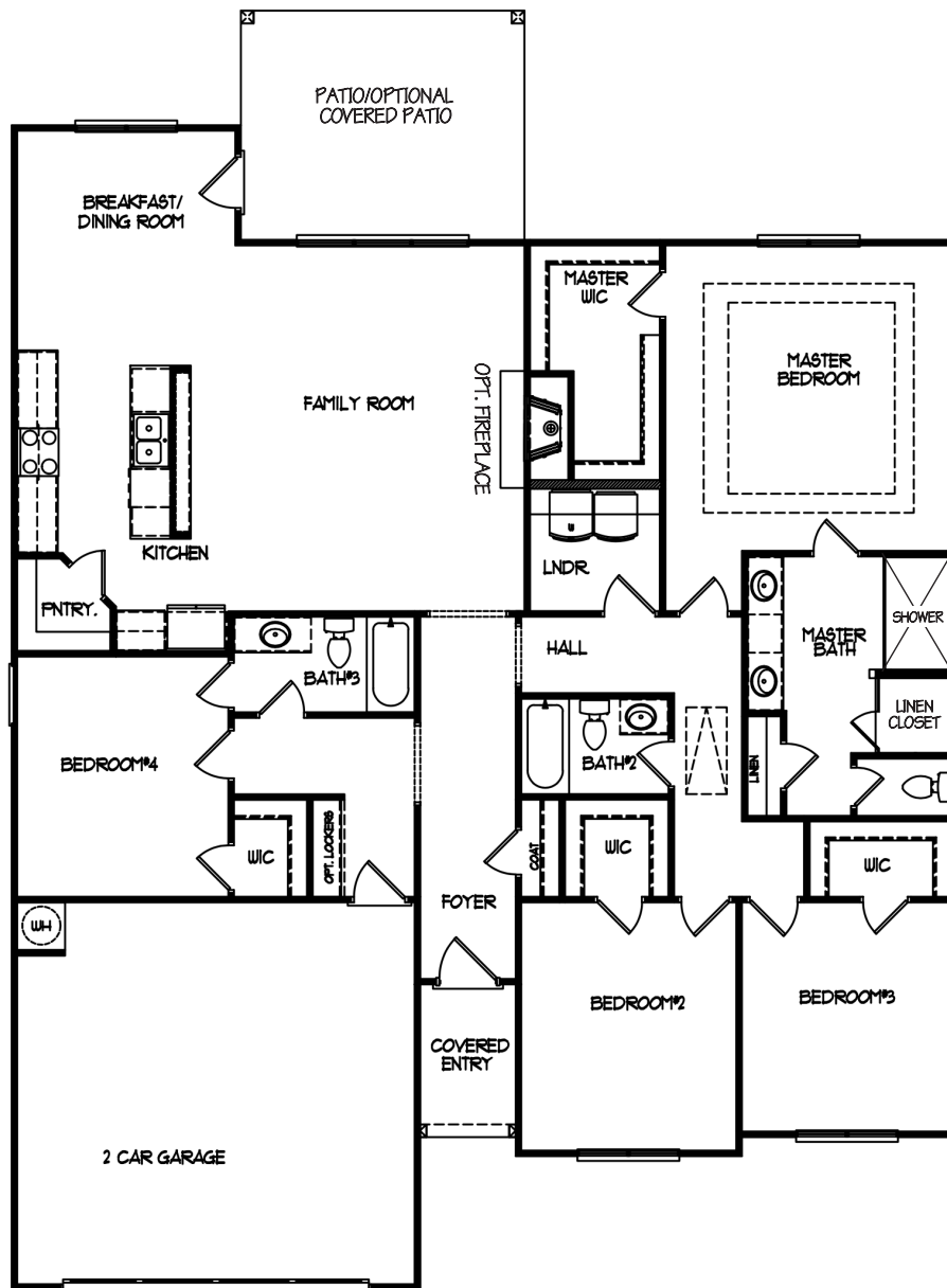
MAIN FLOOR
