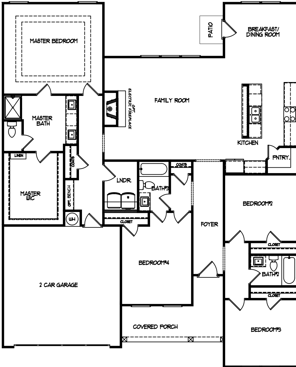
MAIN FLOOR
