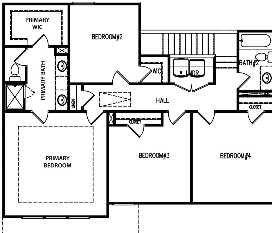
OPT. PRIMARY BATH SUPER SHOWER
