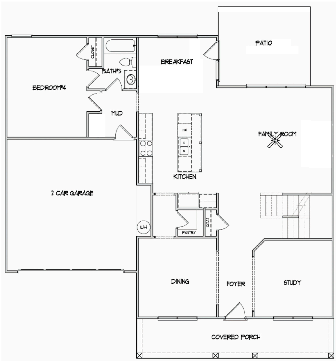
MAIN FLOOR
