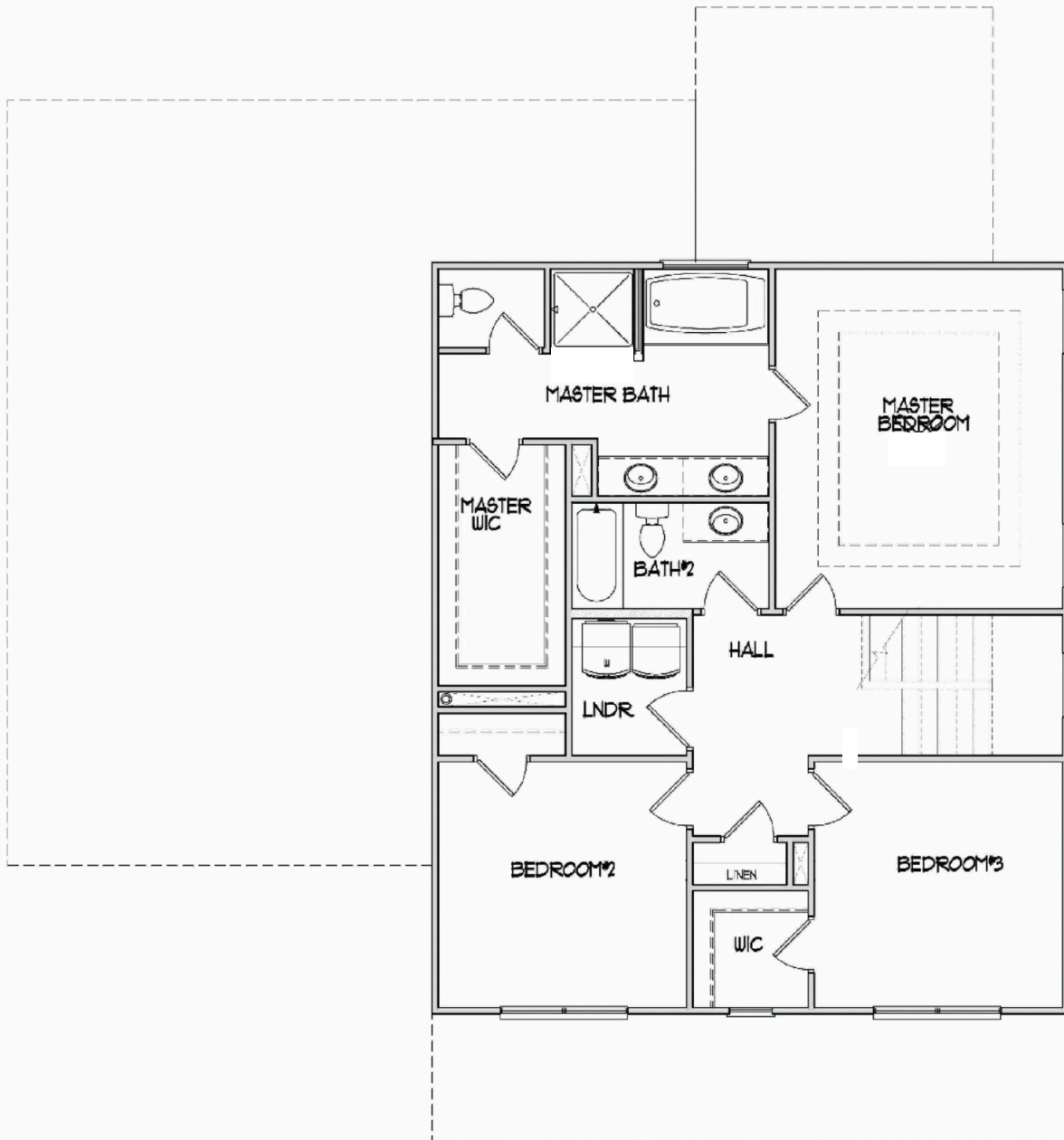
SECOND FLOOR
