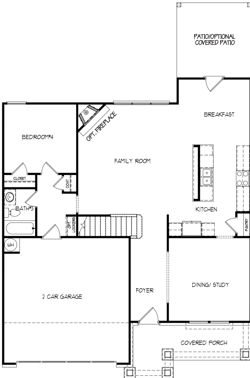
MAIN FLOOR
