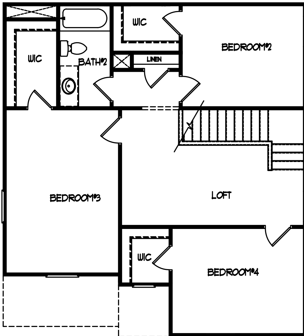
SECOND FLOOR
