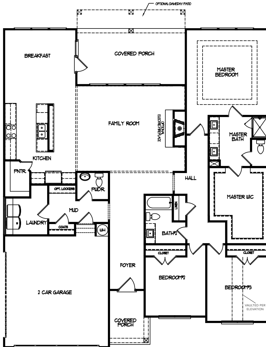
MAIN FLOOR
